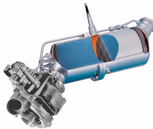
Particulate filter
