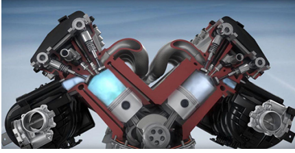
Cylinder deactivation
