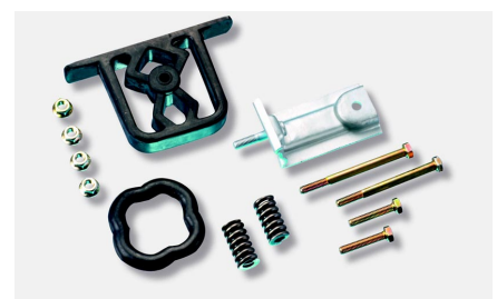
Assembly parts
